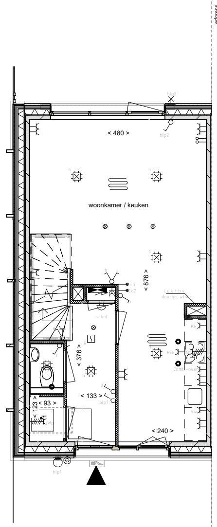
00 begane grond
